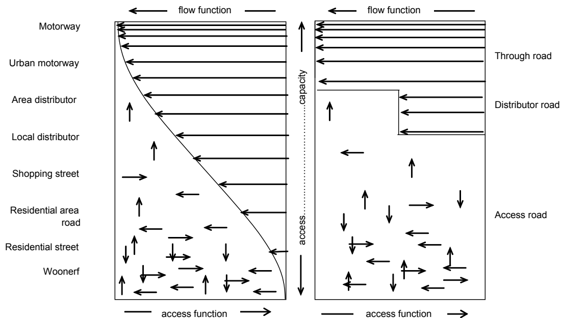
Figure 1. Categorization of roads and streets by access and flow function: on the left according to Goudappel & Perlot (1965) and according to Sustainable Safety on the right.
